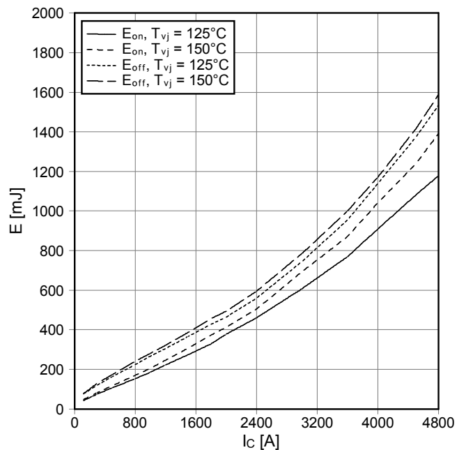
Schaltverluste IGBT-Wechselr. (typisch) switching losses IGBT-inverter (typical) E_{on} = f(I_c), E_{off} = f(I_c) V_{GE} = \pm 15\text{ V}, R_{Gon} = 1.5\ \Omega, R_{Goff} = 0.22\ \Omega, V_{CE} = 600\text{ V}
