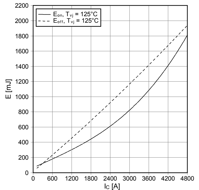
Schaltverluste IGBT-Wechselr. (typisch) switching losses IGBT-inverter (typical) E_{on} = f(I_C), E_{off} = f(I_C) V_{GE} = \pm 15\text{ V}, R_{Gon} = 0.6\ \Omega, R_{Goff} = 0.8\ \Omega, V_{CE} = 900\text{ V}
