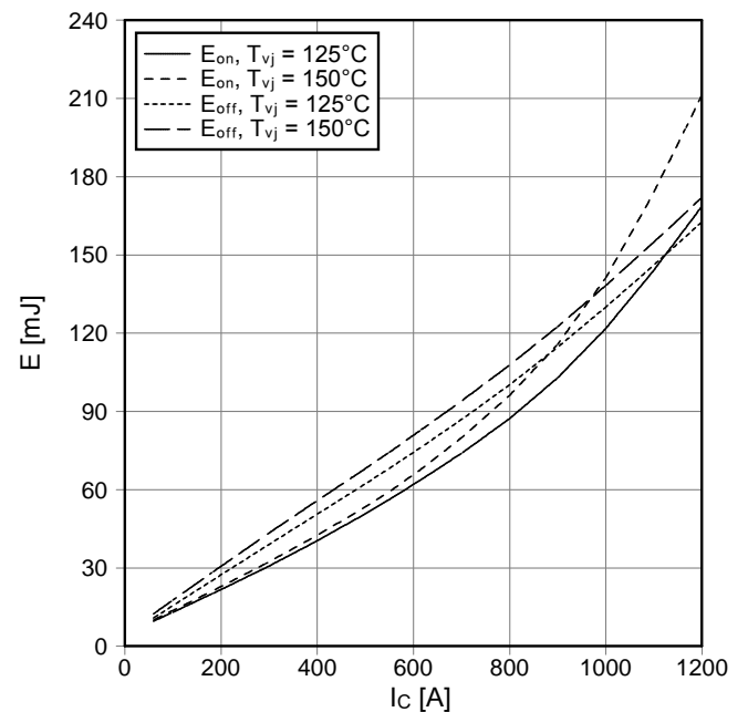
Schaltverluste IGBT-Wechselr. (typisch) switching losses IGBT-inverter (typical) E_{on} = f(I_C), E_{off} = f(I_C) V_{GE} = \pm 15\text{ V}, R_{Gon} = 1.8\ \Omega, R_{Goff} = 2.2\ \Omega, V_{CE} = 600\text{ V}
