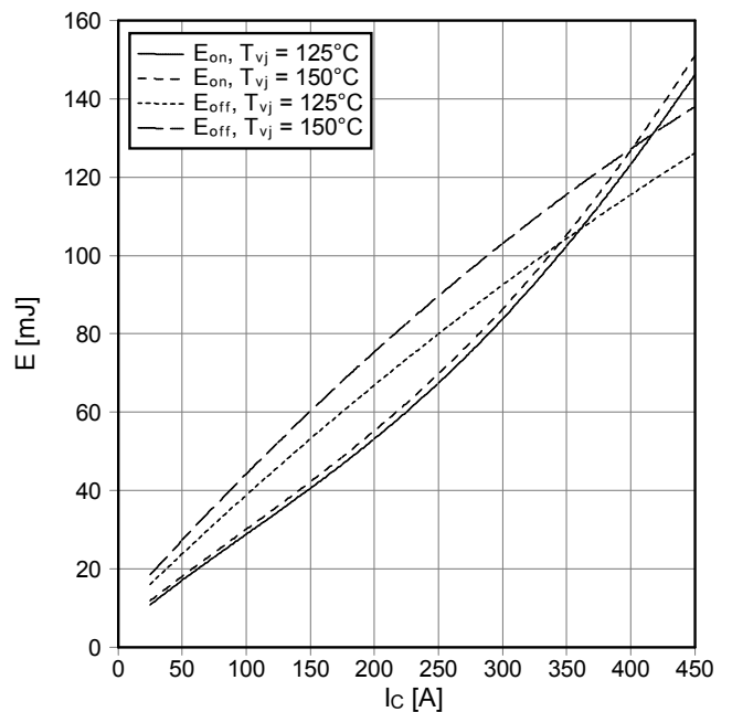
Schaltverluste IGBT-Wechselr. (typisch) switching losses IGBT-inverter (typical) E_{on} = f(I_c), E_{off} = f(I_c) V_{GE} = \pm 15\text{ V}, R_{Gon} = 1.8\ \Omega, R_{Goff} = 1.8\ \Omega, V_{CE} = 900\text{ V}
