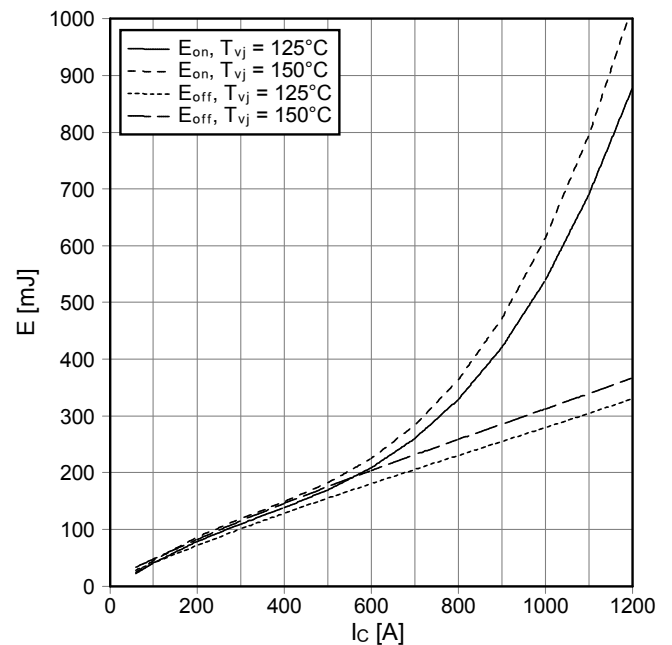
Schaltverluste IGBT-Wechselr. (typisch) switching losses IGBT-inverter (typical) E_{on} = f(I_c), E_{off} = f(I_c) V_{GE} = \pm 15\text{ V}, R_{Gon} = 1\ \Omega, R_{Goff} = 1\ \Omega, V_{CE} = 900\text{ V}
