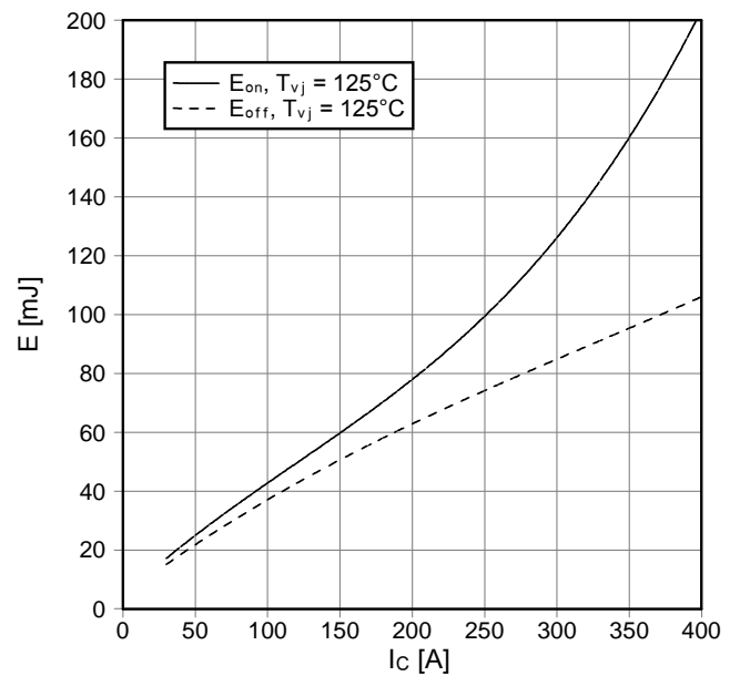
Schaltverluste IGBT-Wechselr. (typisch) switching losses IGBT-inverter (typical) E_{on} = f(I_C), E_{off} = f(I_C) V_{GE} = \pm 15\text{ V}, R_{Gon} = 6,8\ \Omega, R_{Goff} = 6,8\ \Omega, V_{CE} = 900\text{ V}
