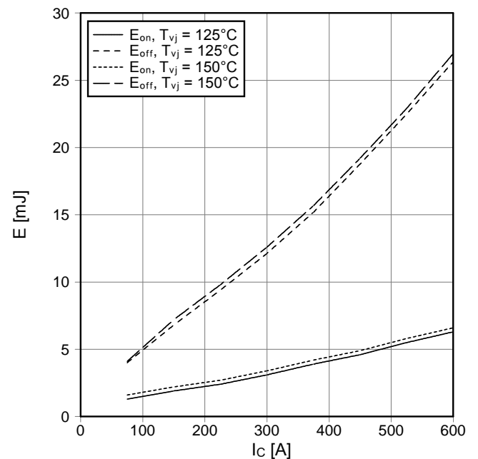
Schaltverluste IGBT-Brems-Chopper switching losses IGBT-brake-chopper E_{on} = f(I_C) , E_{off} = f(I_C) V_{GE} = \pm 15\text{ V} , R_{Gon} = 2.4\ \Omega , R_{Goff} = 2.4\ \Omega , V_{CE} = 300\text{ V}
