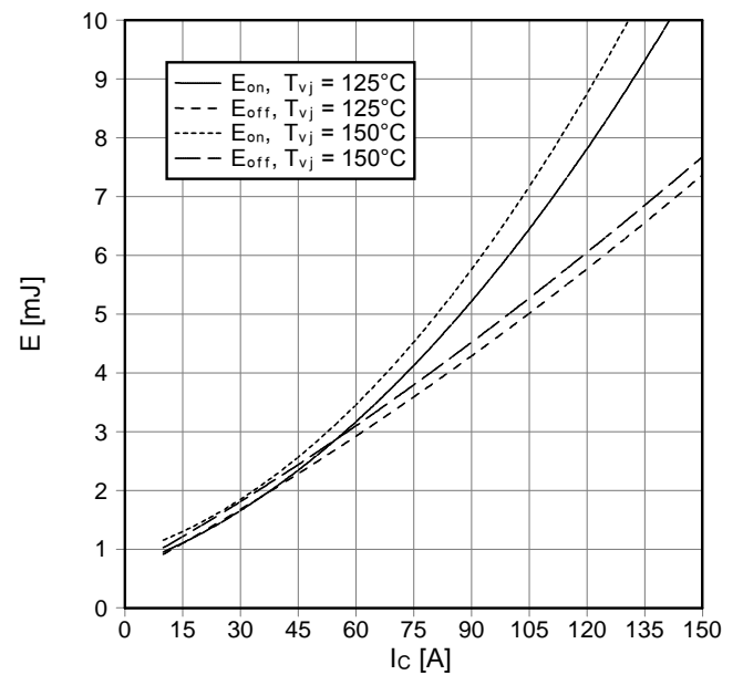
Schaltverluste IGBT-Wechselr. (typisch) switching losses IGBT-inverter (typical) E_{on} = f(I_C) , E_{off} = f(I_C) V_{GE} = \pm 15\text{ V} , R_{Gon} = 30\ \Omega , R_{Goff} = 30\ \Omega , V_{CE} = 300\text{ V}
