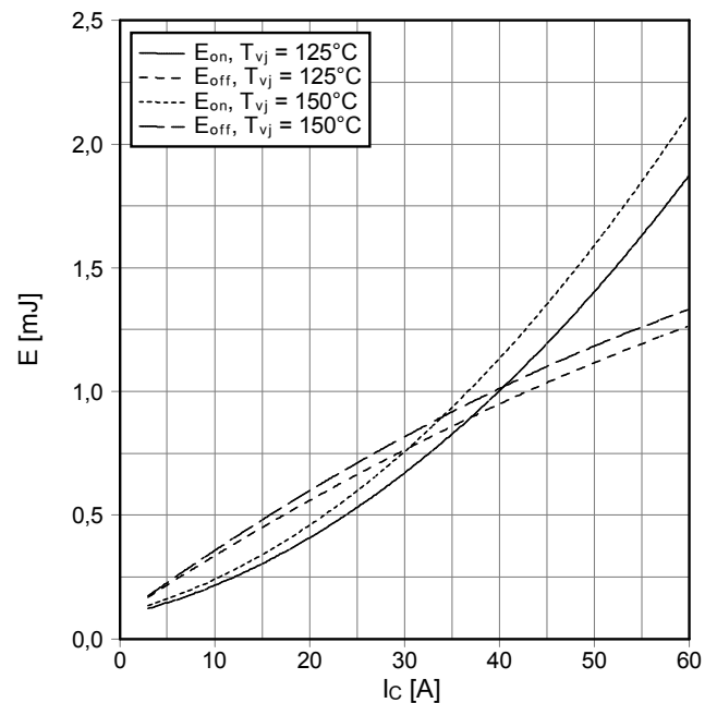
Schaltverluste IGBT-Wechselr. (typisch) switching losses IGBT-inverter (typical) E_{on} = f(I_c) , E_{off} = f(I_c) V_{GE} = \pm 15\text{ V} , R_{Gon} = 15\ \Omega , R_{Goff} = 15\ \Omega , V_{CE} = 300\text{ V}
