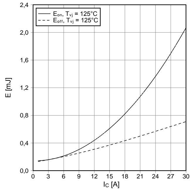
Schaltverluste IGBT-Wechselr. (typisch) switching losses IGBT-inverter (typical) E_{on} = f(I_C) , E_{off} = f(I_C) V_{GE} = \pm 15\text{ V} , R_{Gon} = 68\ \Omega , R_{Goff} = 68\ \Omega , V_{CE} = 300\text{ V}
