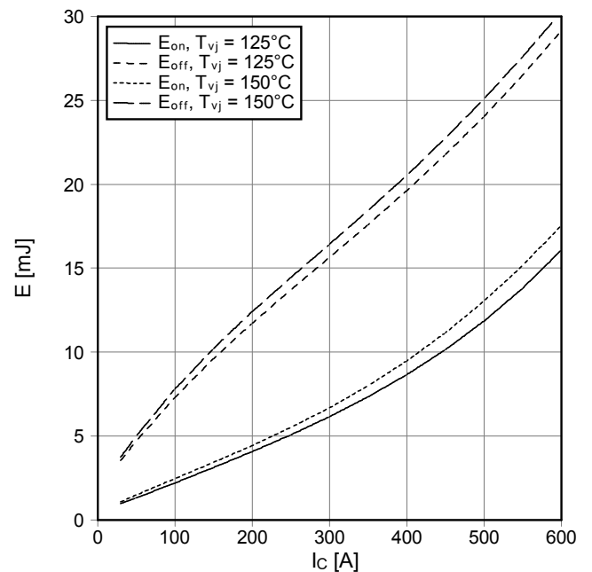
Schaltverluste IGBT-Wechselr. (typisch) switching losses IGBT-inverter (typical) E_{on} = f(I_c), E_{off} = f(I_c) V_{GE} = \pm 15\text{ V}, R_{Gon} = 2.2\ \Omega, R_{Goff} = 1.5\ \Omega, V_{CE} = 300\text{ V}
