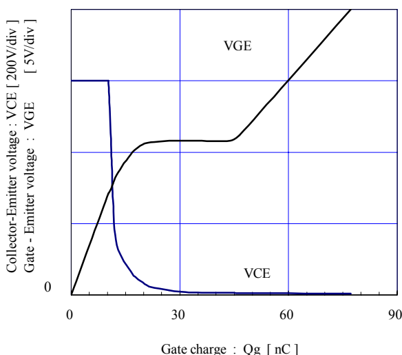
[ Inverter ] Dynamic Gate charge (typ.) Vcc=600V, Ic=25A, Tj= 25°C
