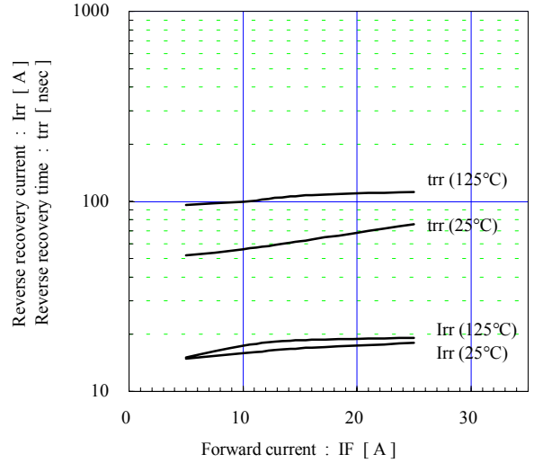
Ⓐ Reverse recovery characteristics (typ.) V_{CC}=600V, V_{GE}=\pm 15V, R_g=68\Omega
