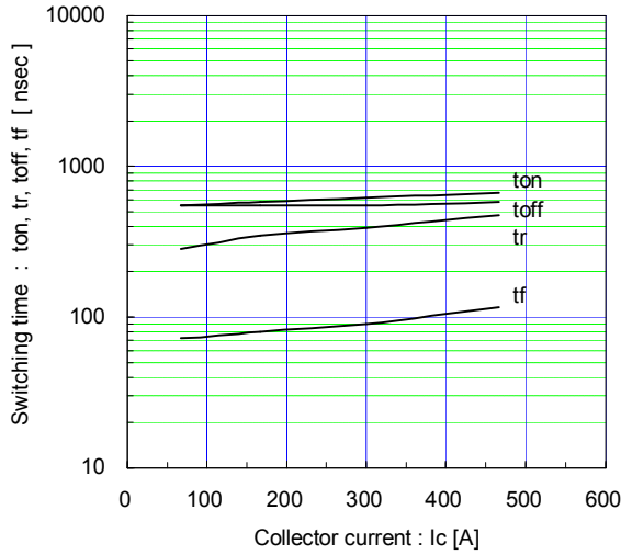
Switching time vs. Collector current (typ.) V_{cc}=900V, V_{GE}=\pm 15V, R_g=1.5\Omega, T_j=25^\circ C
