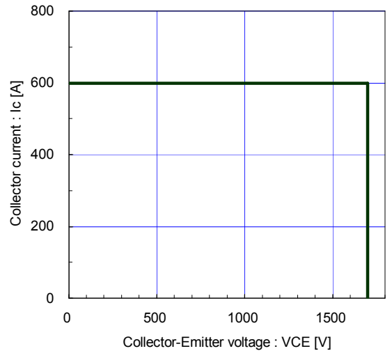
Reverse bias safe operating area (max.) +V_{GE}=15V, -V_{GE} \le 15V, R_g \ge 1.5\Omega, T_j \le 125^\circ C Stray inductance \le 100nH
