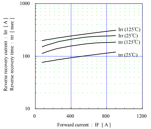
Reverse recovery characteristics (typ.) Vcc=300V, VGE=±15V, Rg=4.7Ω
