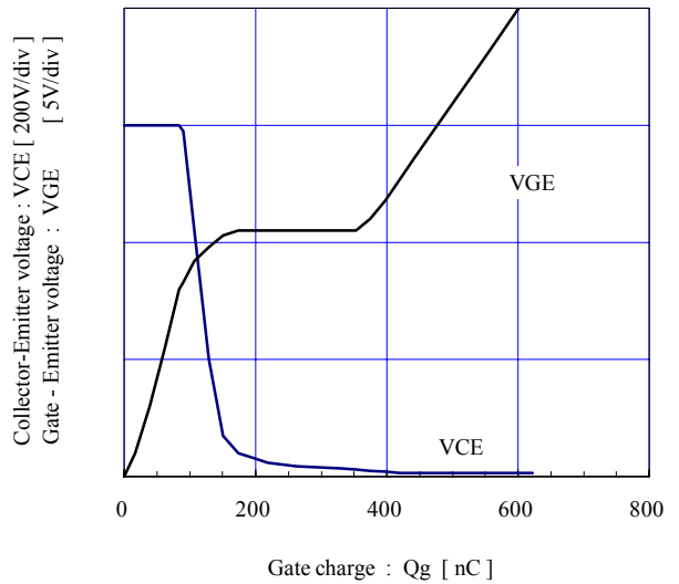
Dynamic Gate charge (typ.) Vce=300V, Ic=150A, Tj= 25°C
