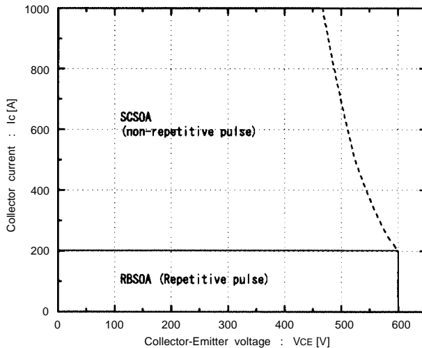
Reversed biased safe operating area +V_{GE}=15V, -V_{GE} \le 15V, T_j \le 125^\circ C, R_G \ge 24\text{ ohm}
