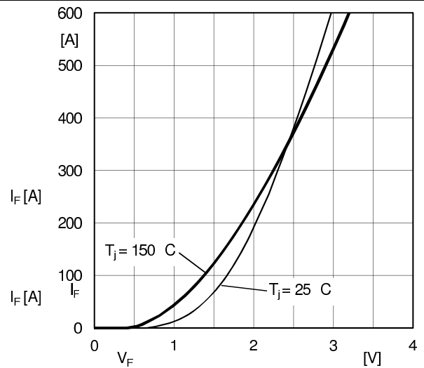
Fig. 10: Typ. CAL diode forward charact., incl. R_{CC+EE}
